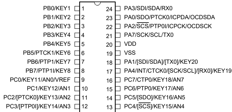
BS86D20C/BS86DV20C 24 SOP-A
