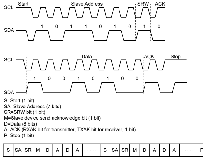
I 2 C Communication Timing Diagram
