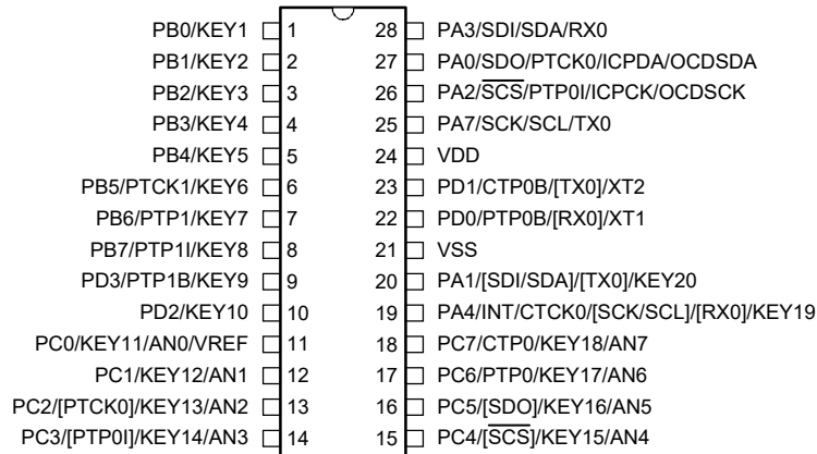
BS86D20C/BS86DV20C 28 SOP-A
