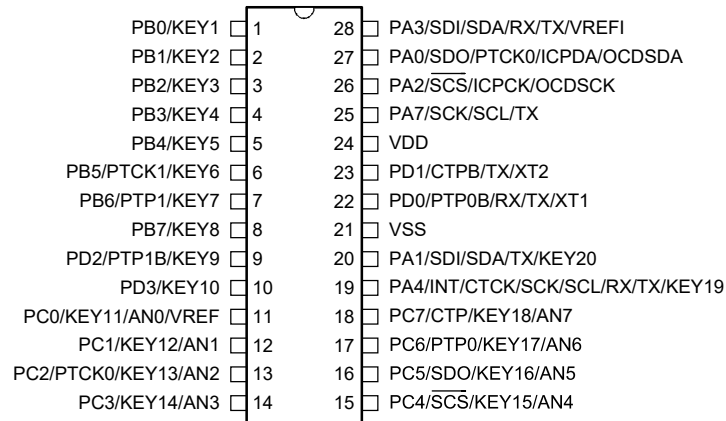
BS86D20CA/BS86DV20CA 28 SOP-A/SSOP-A
