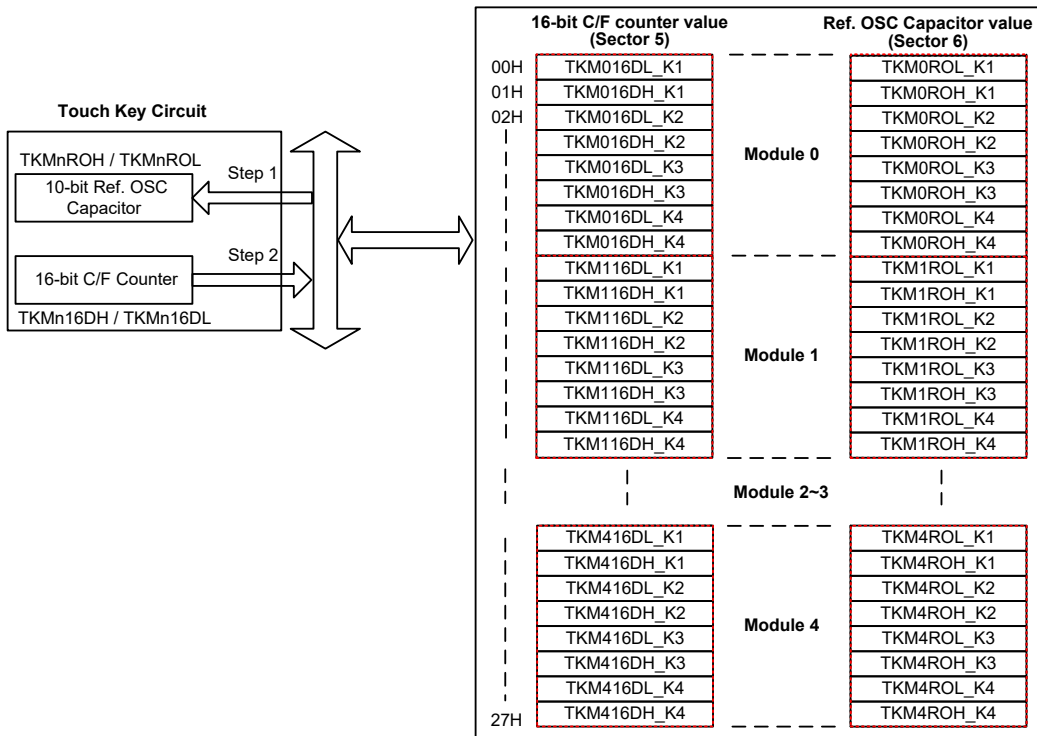
Touch Key Module Data Memory Map
