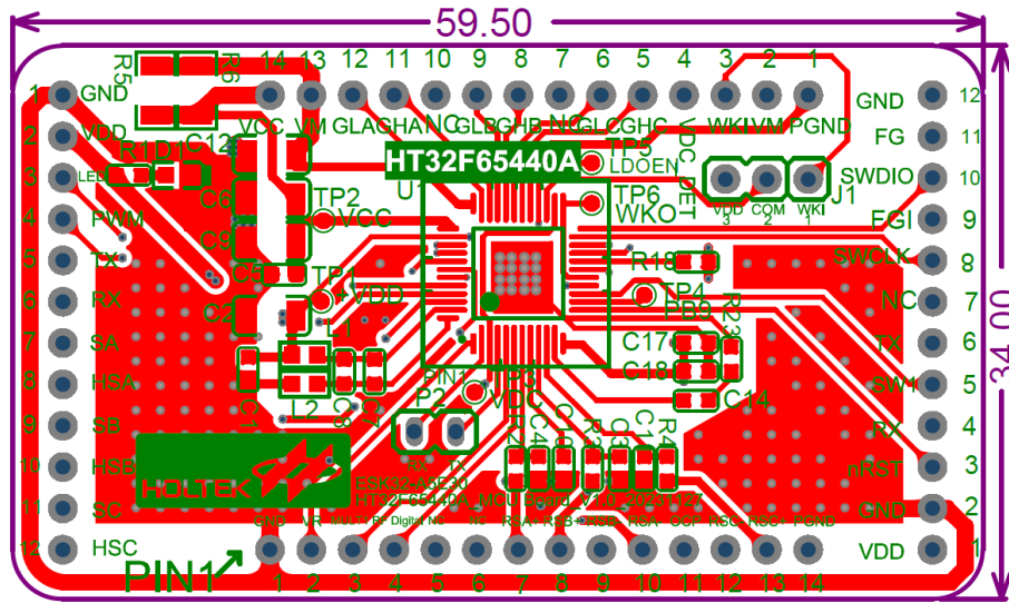
HT32F65440A_MCU Board_Top Layer
