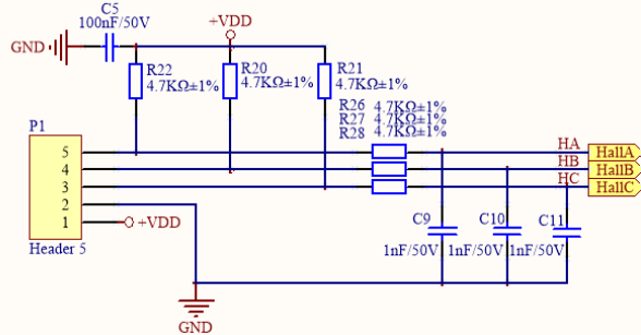
Hall Sensor Feedback Circuit
