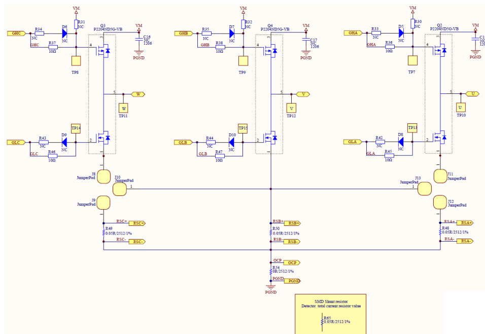
Inverter Circuit
