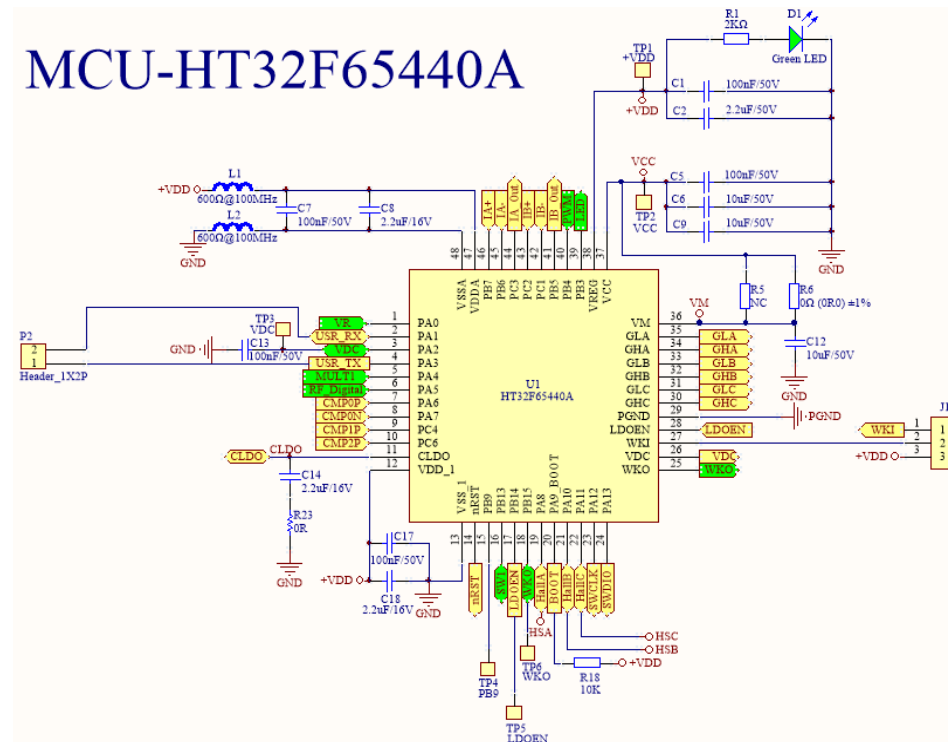
HT32F65440A Peripheral Component Reference Circuit
