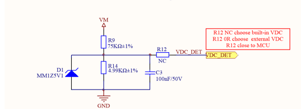
DC Bus Voltage Feedback Circuit
