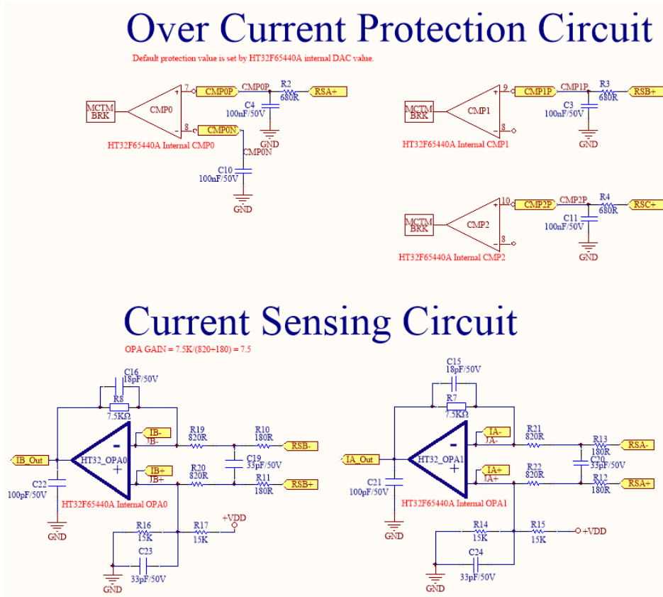
Over Current Protection Circuit and Current Sensing Circuit
