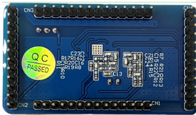
BLDC Motor Workshop HT32F65440A_MCU Board Back View
