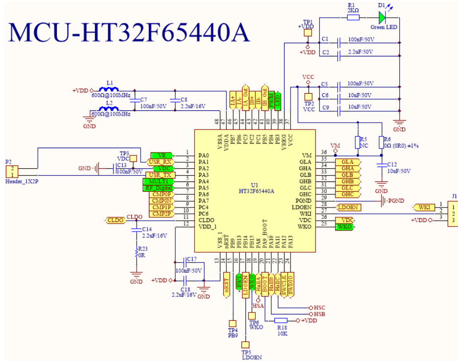
HT32F65440A Pin Circuit Diagram
