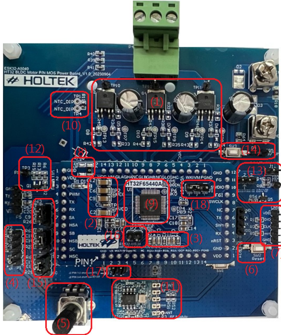
BLDC Motor Workshop HT32F65440A_MCU Board and HT32 BLDC Motor P/N MOS Power Board Front View
