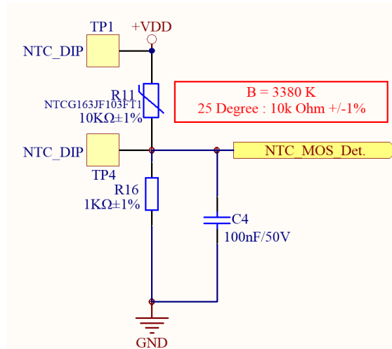
MOSFET Temperature Feedback Circuit
