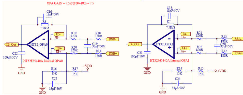
OPA Circuit of Phase Current Sampling
