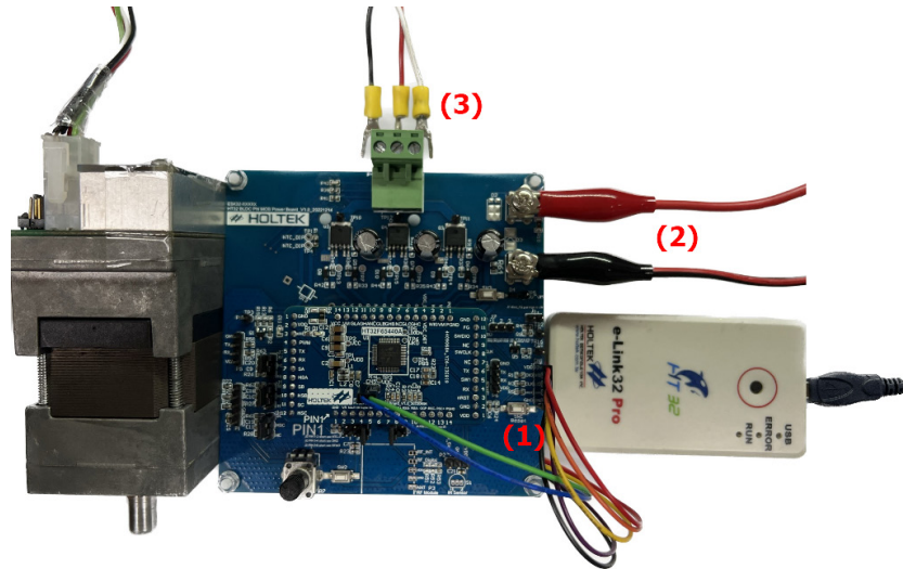
Check the HT32F65440A_MCU Board and the HT32 BLDC Motor P/N MOS Power Board Hardware Pre-setting Wiring
