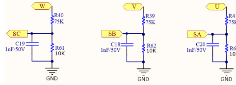
Back EMF Detection Circuit
