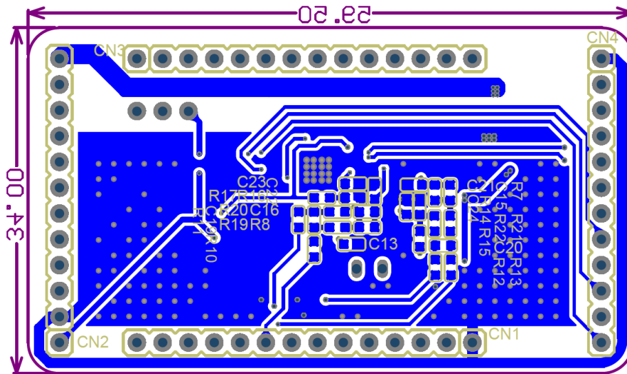
HT32F65440A_MCU Board_Bottom Layer
