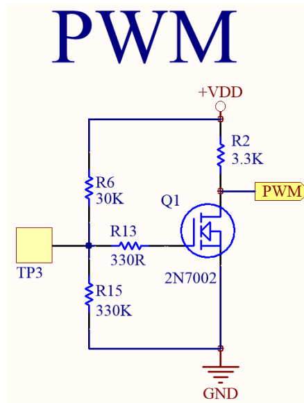
PWM Command Function
