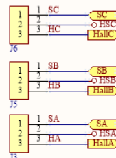
Sensorless and Hall Sensor Jumper Settings
