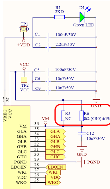
R5 and R6 Buck Resistors
