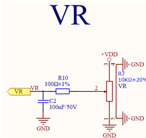
VR Variable Resistor Circuit
