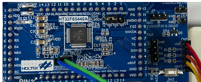
HT32F65440A_MCU Board P2 and HT32 BLDC Motor P/N MOS Power Board CN5 Corresponding Programming Cable Color Reference
