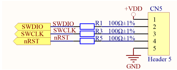
CN5 Pin Definition
