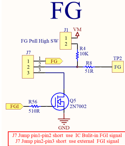
FG Speed Function
