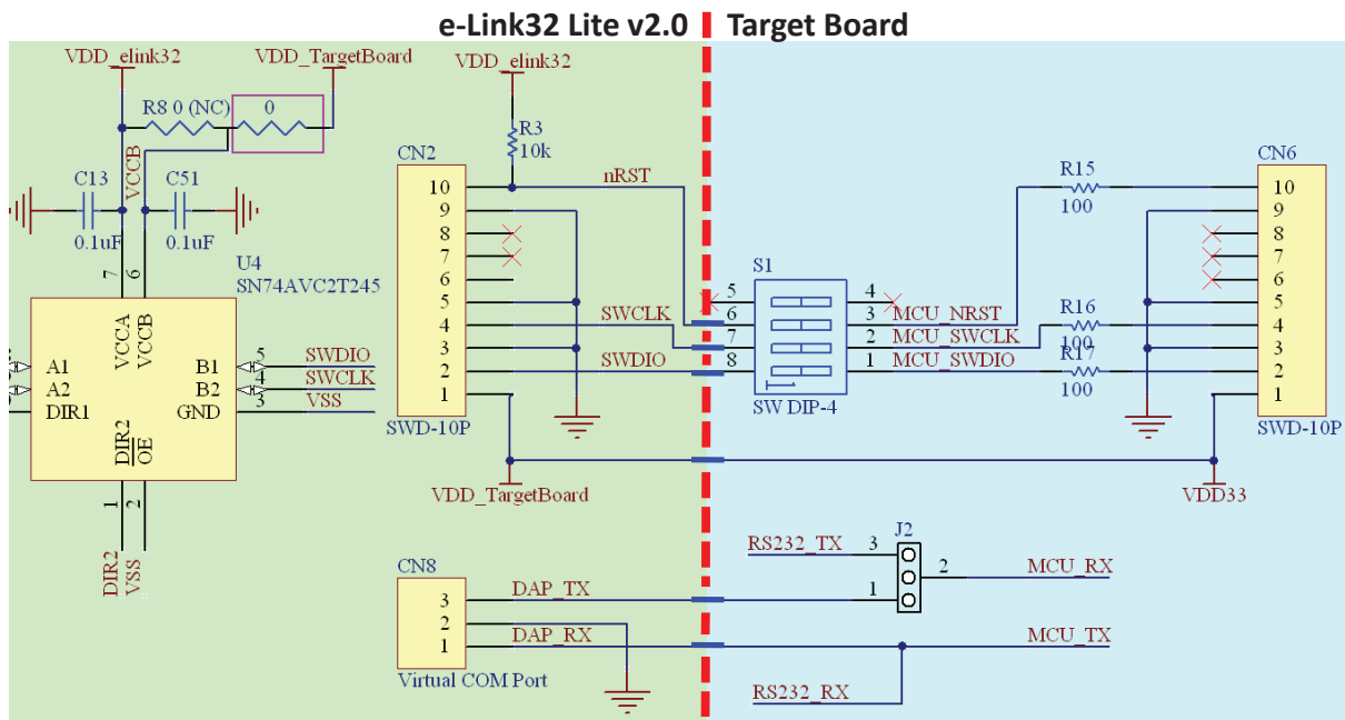
Figure 8. Connection between the e-Link32 Lite V2.0 and the Target Board
