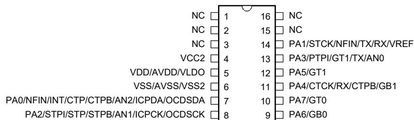
HT45F4840/HT45V4840 16 NSOP-A
