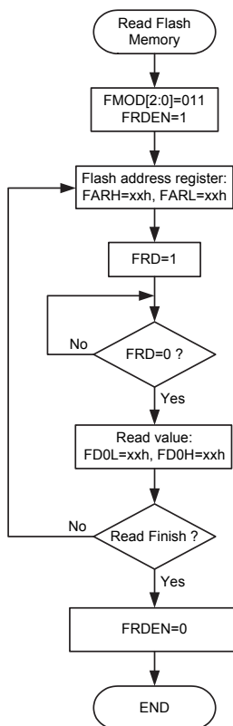
Flash Memory Read Procedure
