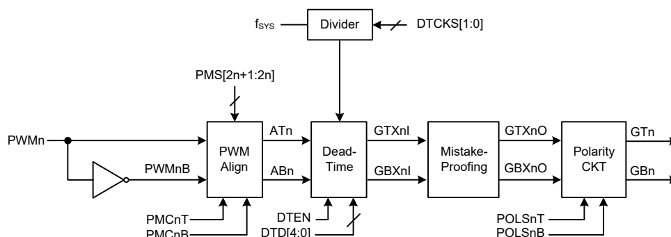
Complementary PWM Output Control Block Diagram (n=0~1)
