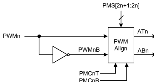
PWM Align Block Diagram (n=0~1)
