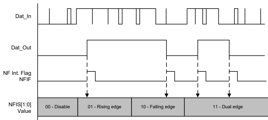
Digital Noise Filter Timing
