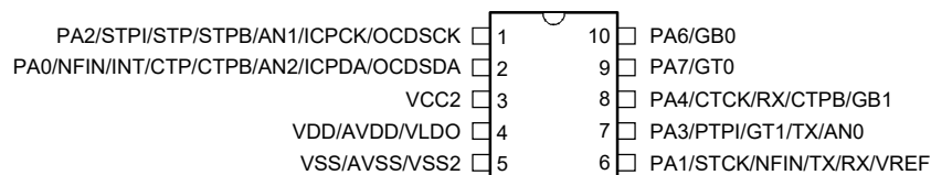
HT45F4840/HT45V4840 10 SOP-A
