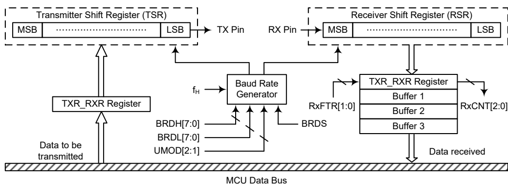
UART Data Transfer Block Diagram
