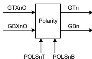
Polarity Control Block Diagram (n=0~1)
