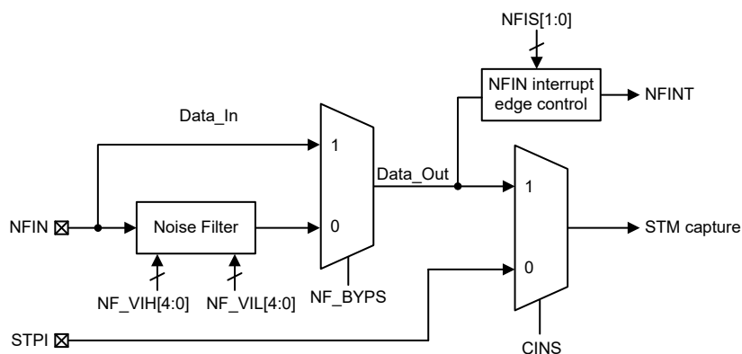
Digital Noise Filter Block Diagram
