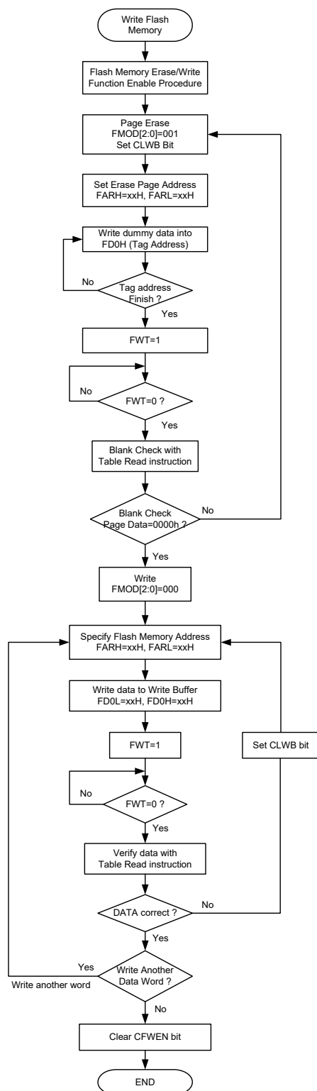
Flash Memory Non-Consecutive Write Procedure
