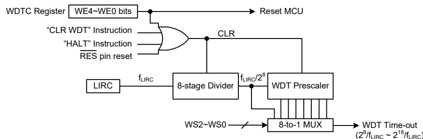
Watchdog Timer
