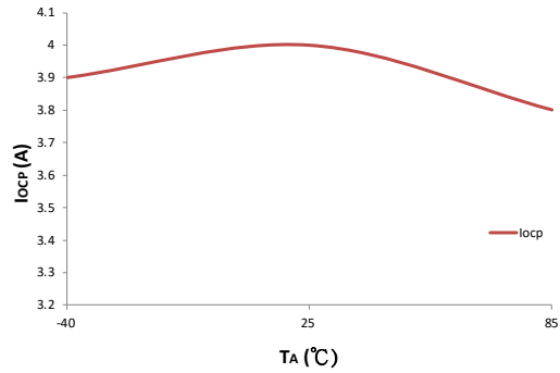
I_{OCP} vs. Temperature
