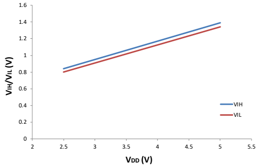
V_{IH}/V_{IL} vs. V_{DD}
