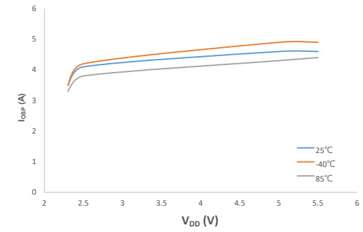
I_{OSR} vs V_{DD} Characteristics
