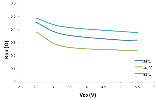
R_{ON} vs. V_{DD} (-40°C, 25°C, 85°C)
