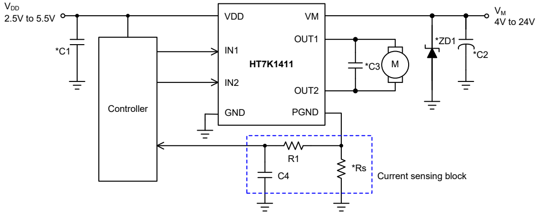
Motor Current Sensing
