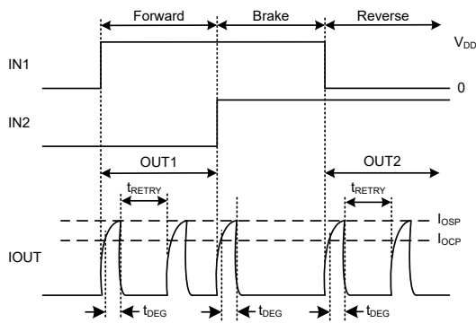
Figure 6. Retry Mechanism
