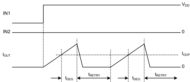
Figure 3. OCP Reaction
