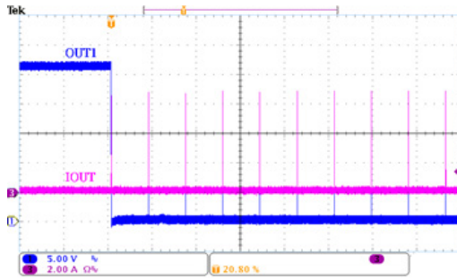
Short Circuit Protection Reaction
