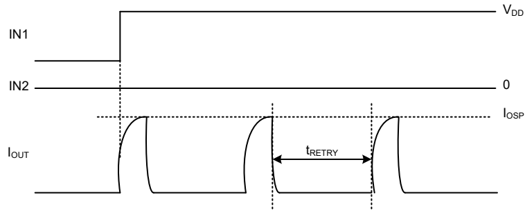
Figure 4. OSP Reaction
