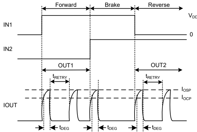
Figure 5. Retry Reaction
