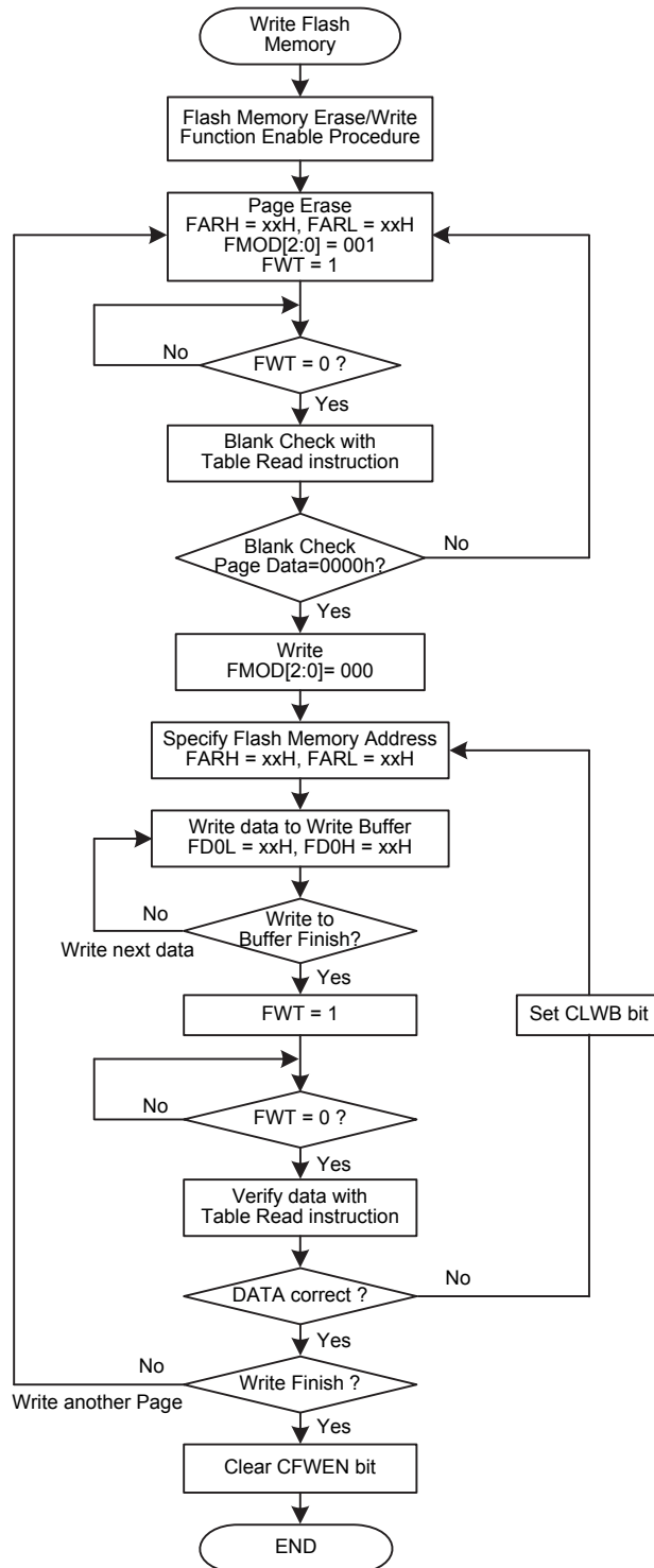
Flash Memory Consecutive Write Procedure
