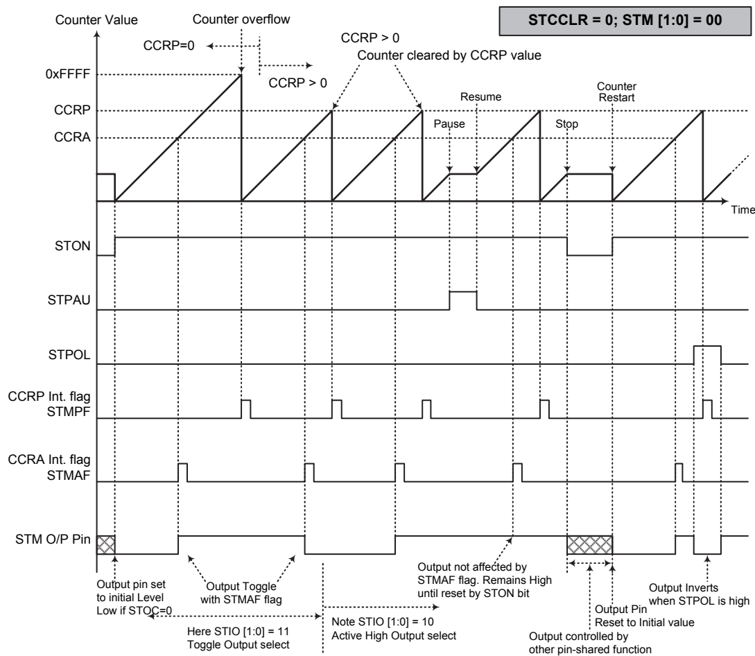
Compare Match Output Mode – STCCLR=0
