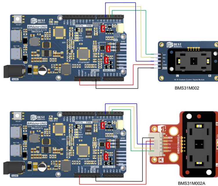
Physical Connection Diagram
