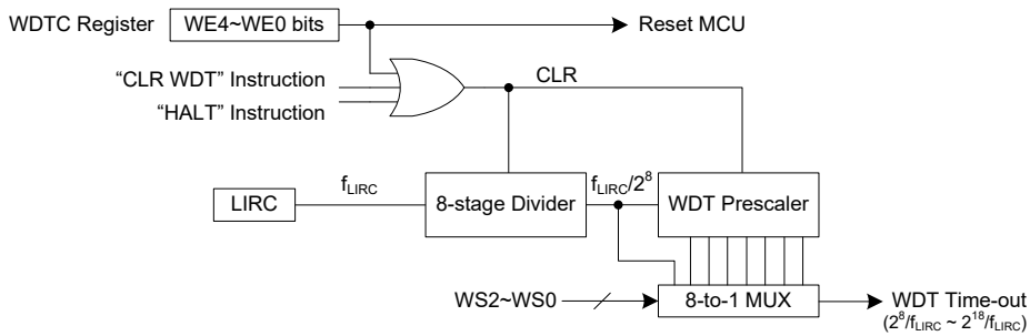
Watchdog Timer
