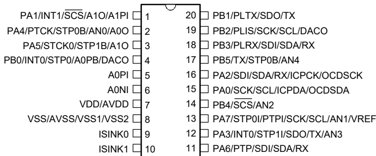
BA45F5250/BA45V5250 20 SSOP-A
