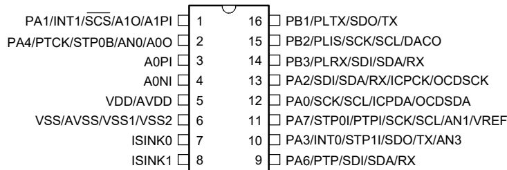
BA45F5250/BA45V5250 16 NSOP-A
