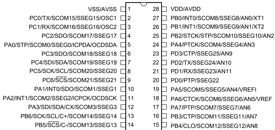
HT66F3195/HT66V3195 28 SSOP-A
