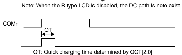
R Type Bias Voltage Configuration – 1/3 Bias (n=0~3)
