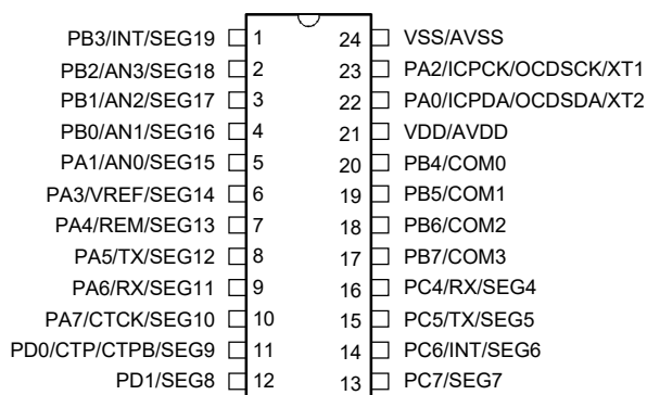
HT67F2432/HT67V2432 24 SOP-A/SSOP-A
