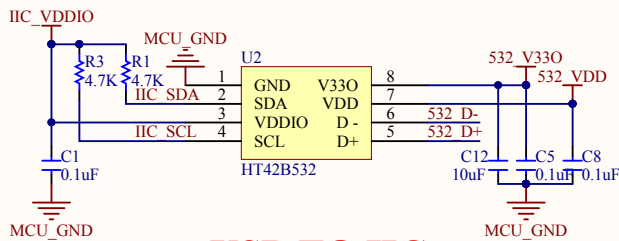
USB TO IIC
