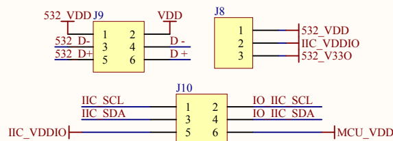
connect to TDS Module
