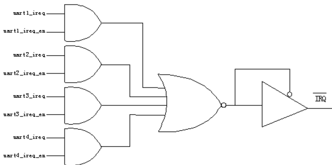
Figure 8.3 WK2124 Interrupt Structure Diagram
