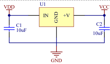
LDO Circuit
